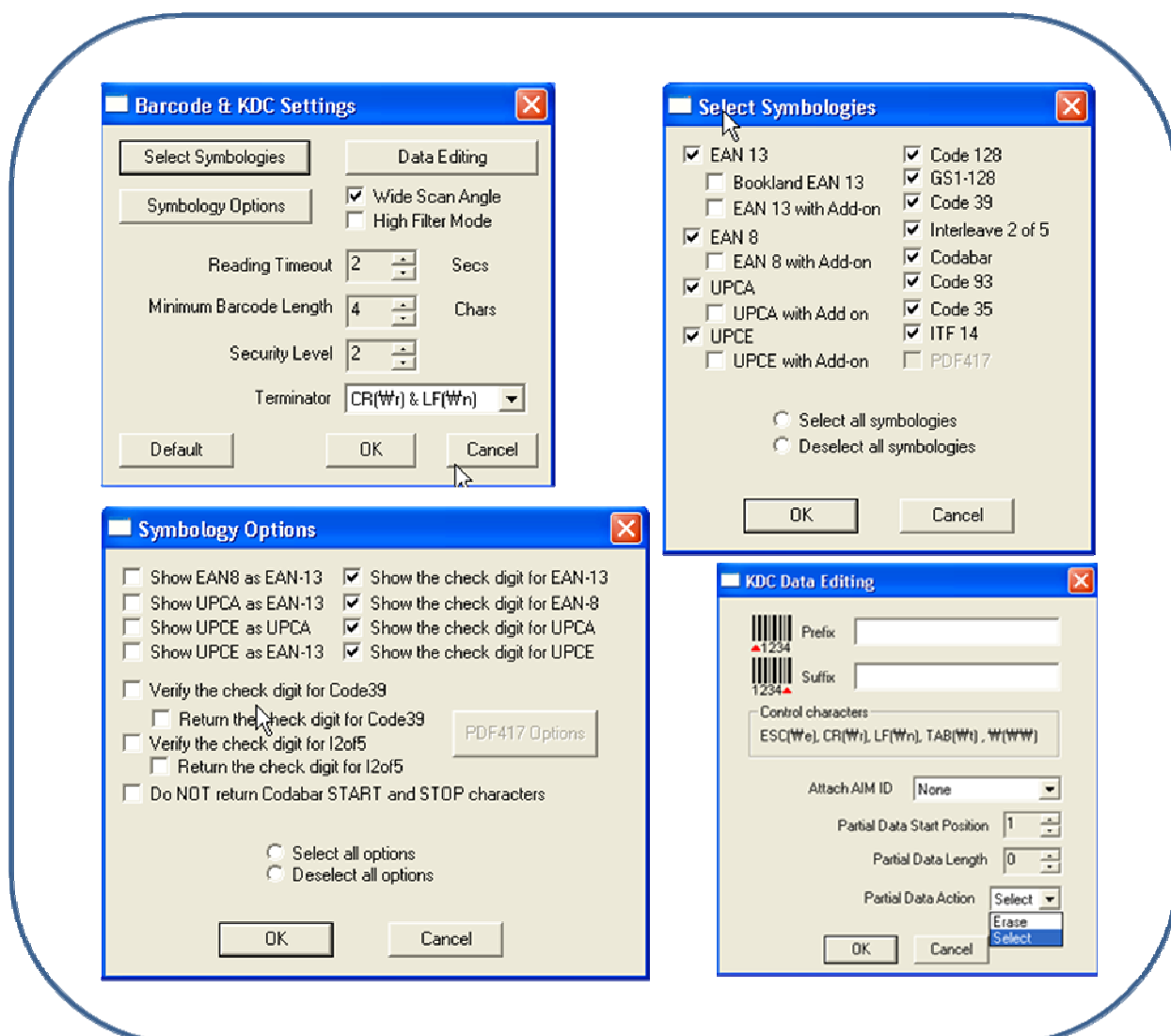
Figure 14 - Barcode & KDC Settings, Symbolgies, Data Editing and Scan Options
