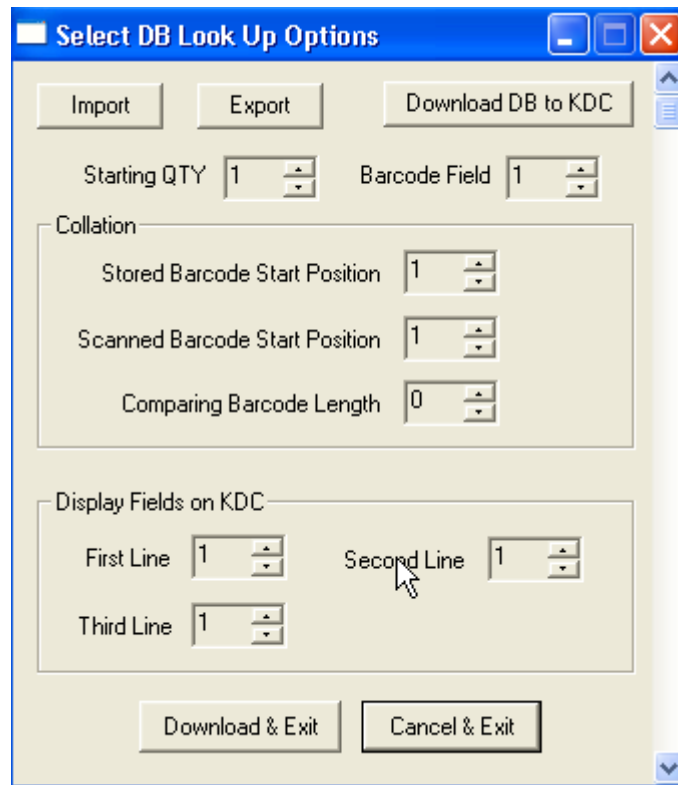
Figure 28 – DB Lookup Application Menu
