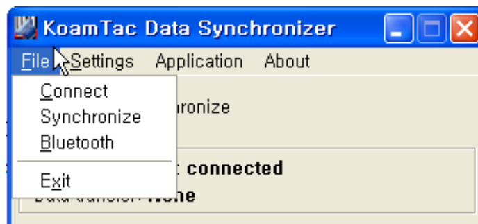
Figure 7 – File Menu
