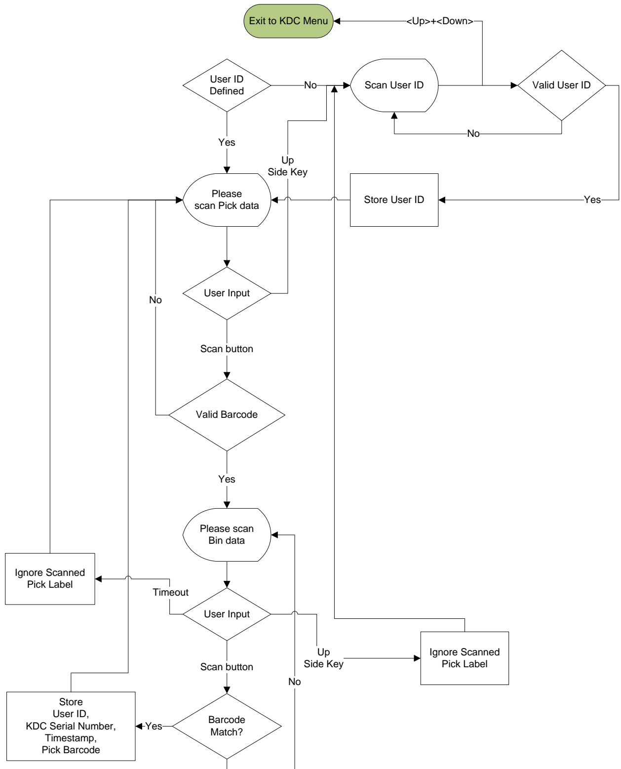
Figure 27 – Pick/BIN Application Flow Chart
