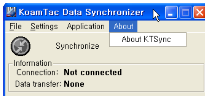
Figure 10 – About Menu
