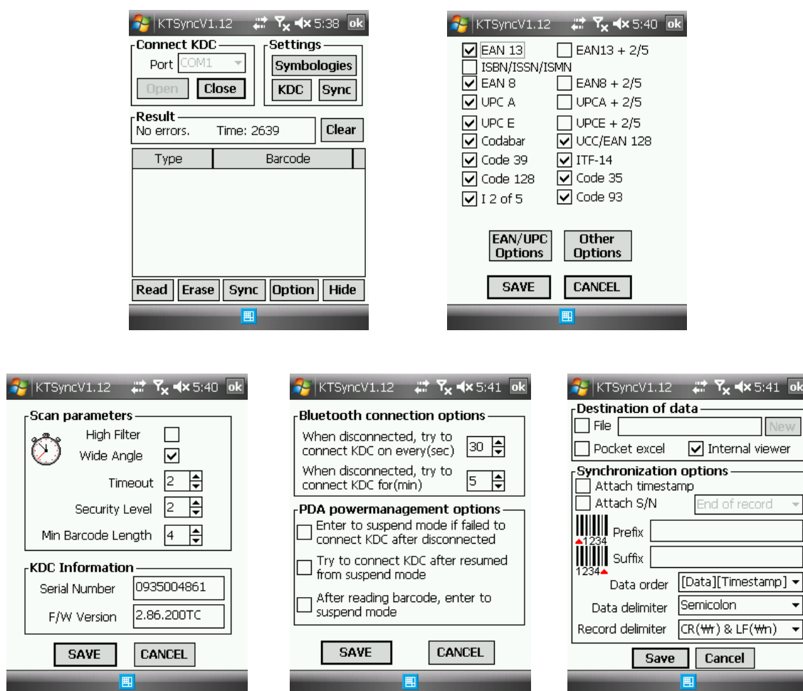
Figure 16 – Mobile pKTSync
