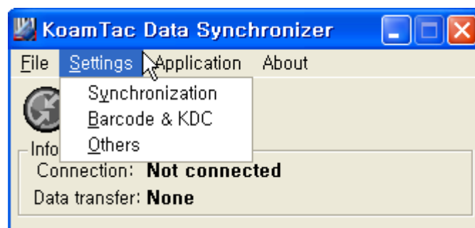
Figure 8 – Setting Menu
