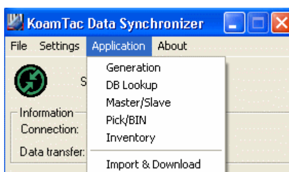
Figure 20 – Application Menu
