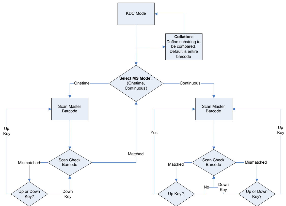
Figure 25 – Master/Slave Application Flow Chart
