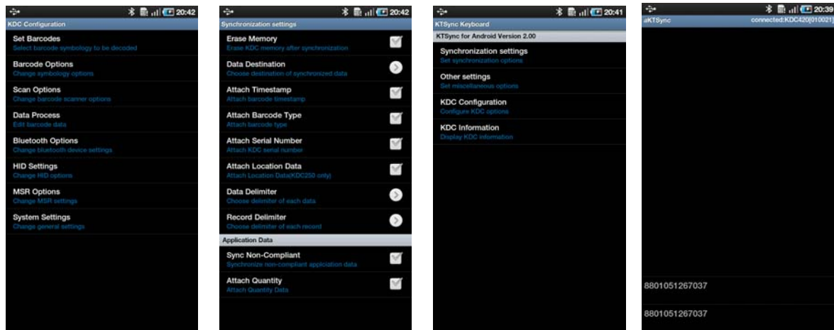
Figure 17 – Android aKTSync
