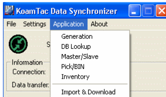
Figure 9 – Application Menu
